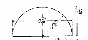
BEARING-BORE GAUGE 3 3/4 x 7 JOURNAL.
